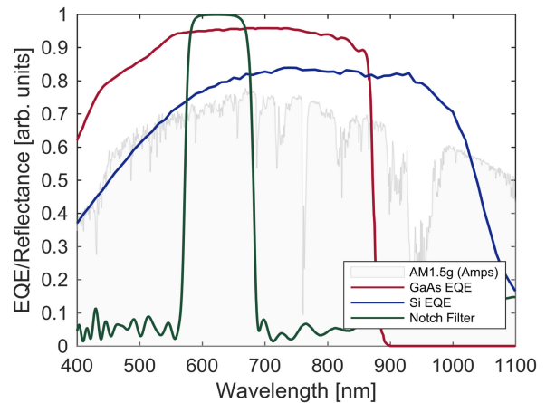
Fig. 4. EQE of the embedded GaAs and underlying IBC Si cells, referenced to the AM1.5G spectrum.
