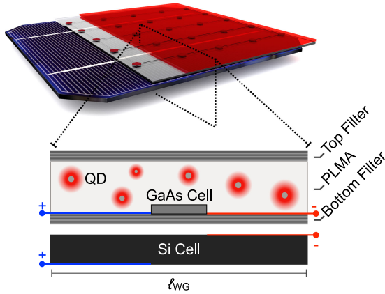
Fig. 2. Conceptual rendering of the tandem LSC/Si module (top) and its cross section (bottom). The cross section shows a single unit cell of the full tandem device architecture, and indicates electrical connections to the top and the bottom cell.
