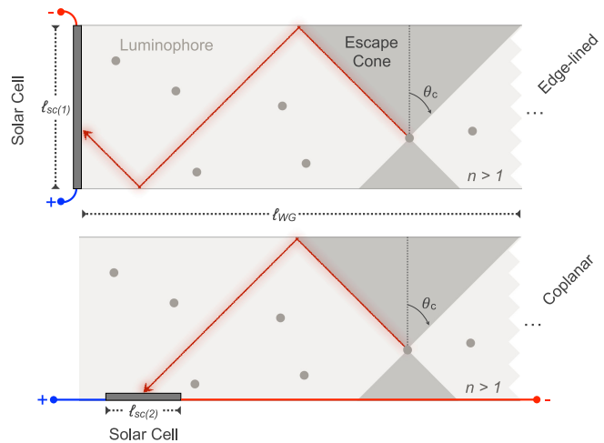
Fig. 1. Two-dimensional schematic of an LSC in the (top) edge lined and (bottom) coplanar orientations of the solar cell. Here, \theta_c is the critical angle of the escape cone.
