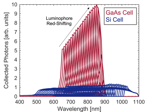
Fig. 7. Increase of collected photocurrent from the GaAs microcells of the tandem LSC/Si for continual redshifting of the QD luminophores up until the band edge.
